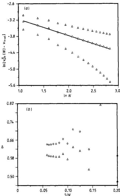
Figure 3. Dependence on \ln N of \ln[\nu_{\text{eff}}^{\text{II}}(N) - \nu_{\text{trial}}] using 'method II' (equation (6)), for the choices \nu_{\text{trial}} = 0.74, 0.75 and 0.76 (top curve). Since the limiting slope is -\Delta , we show in (b) the sequence of slopes obtained by placing a straight line segment through successive pairs of points in (a). Also shown in (b) ( \diamond ) are estimates of \Delta(N) obtained by 'method IV' (equation (8)); these should approach correction-to-scaling exponent \Delta .
