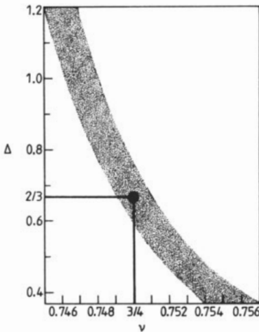
Figure 1. Dependence of the correction-to-scaling exponent \Delta on \nu , the 'trial' value of \nu , showing that even a very small change in \nu leads to a very large change in \Delta . The shaded region indicates the combination of several independent methods of estimating this dependence.
