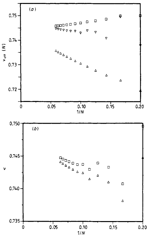
Figure 2. (a) shows the dependence on 1/N of the three sequences of successive approximations \nu_{\text{eff}}^I(N) to the correlation length exponent \nu for the triangular lattice SAW problem. \square , equation (5); \triangle , equation (6); \nabla , equation (7). (b) shows the sequence of intercepts obtained by placing a straight line segment through successive pairs of points in part (a).
